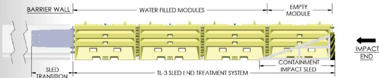
SLED™ TL-3 4900 lb. Pick-Up Truck Impact Attached to Concrete Median Barrier Wall
