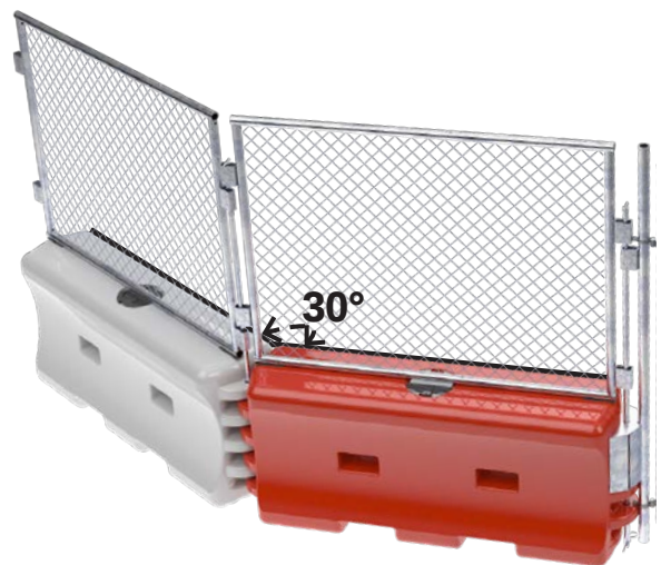
Maximum Rotation With 6ft T-Pin
