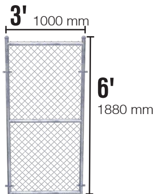
3' Single Gate: 45032-WWF-G3
