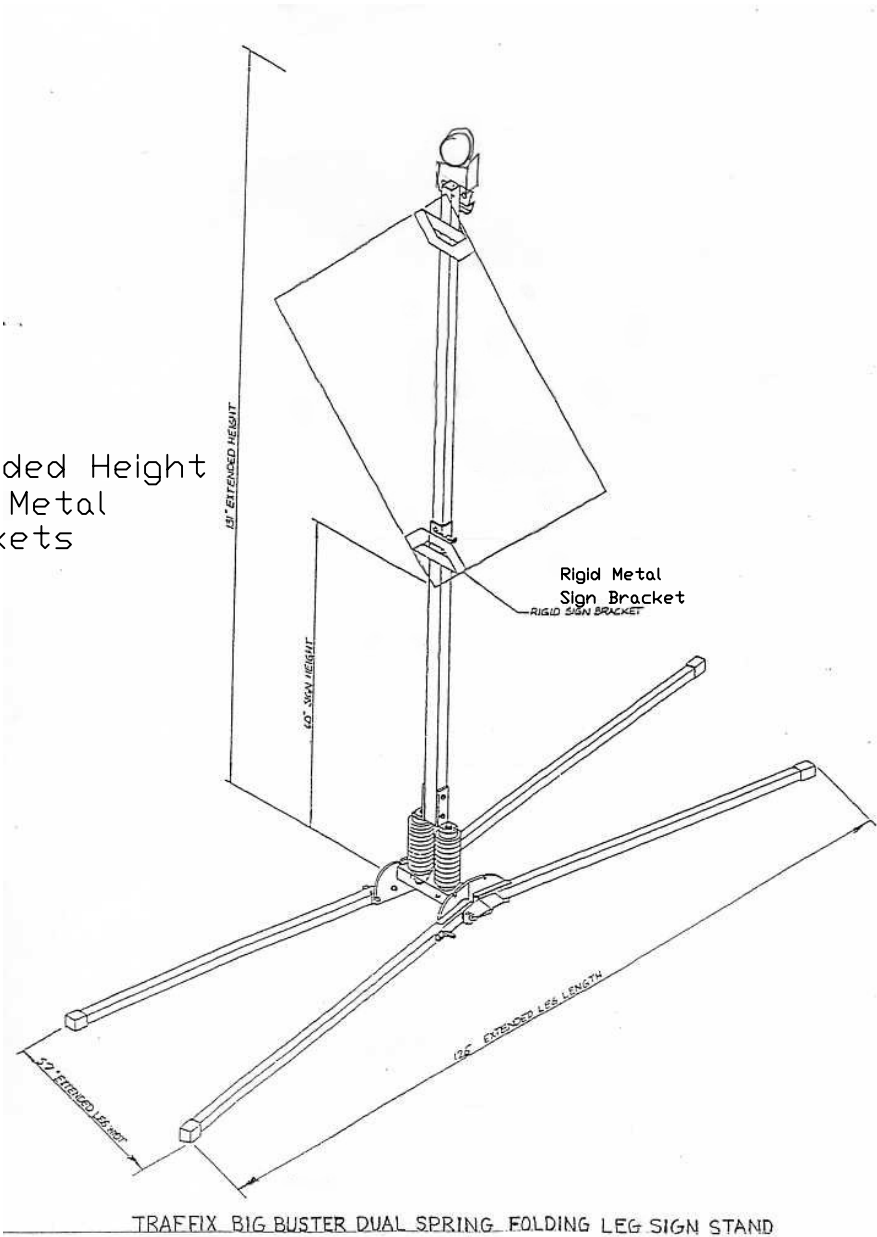
TRAFFIX BIG BUSTER DUAL SPRING FOLDING LEG SIGN STAND WITH RIGID METAL SIGN BRACKETS
